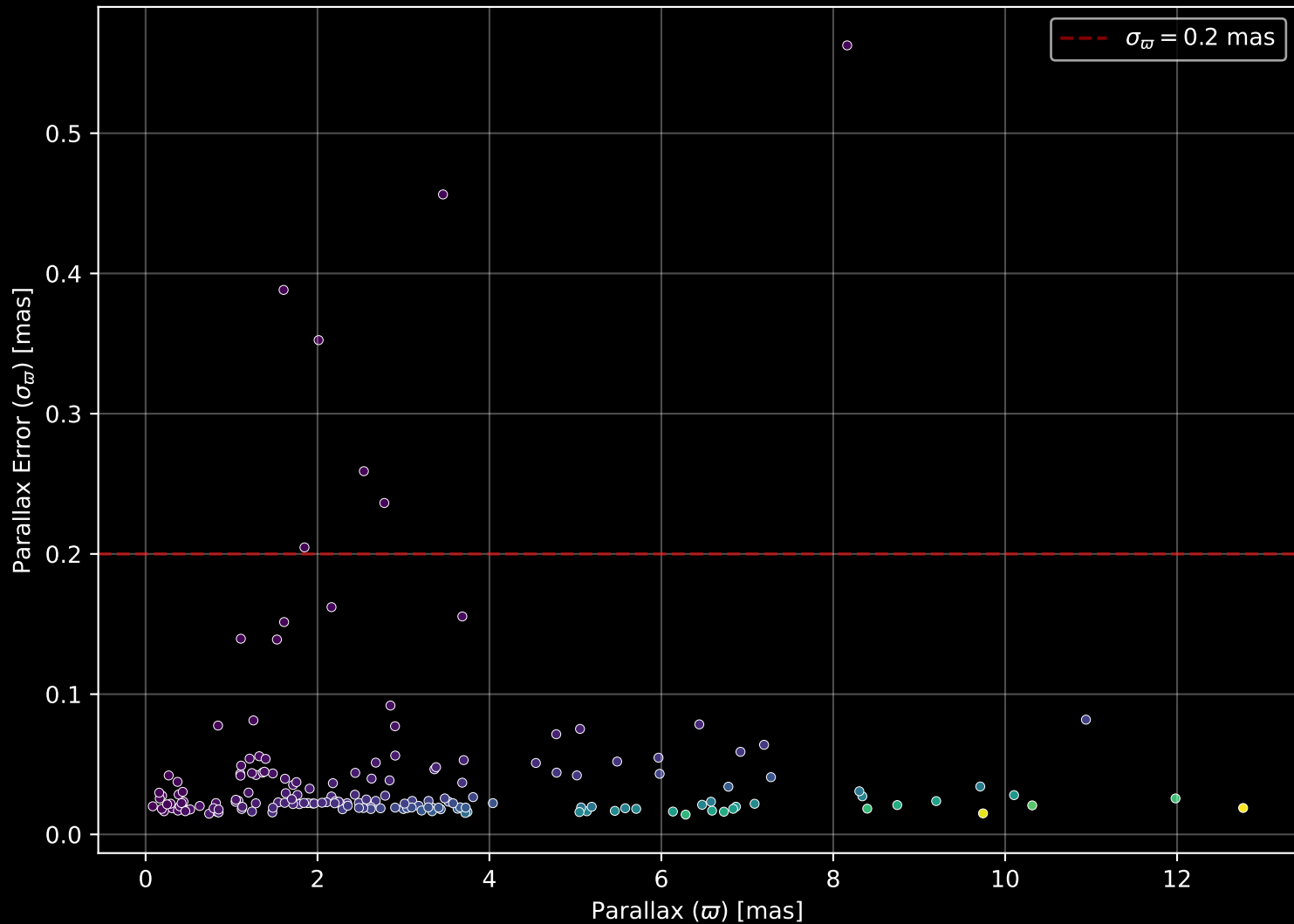
APOGEE DR17 Field: [K2_C8_130-53_btx] Parallax Quality (n= 177)
