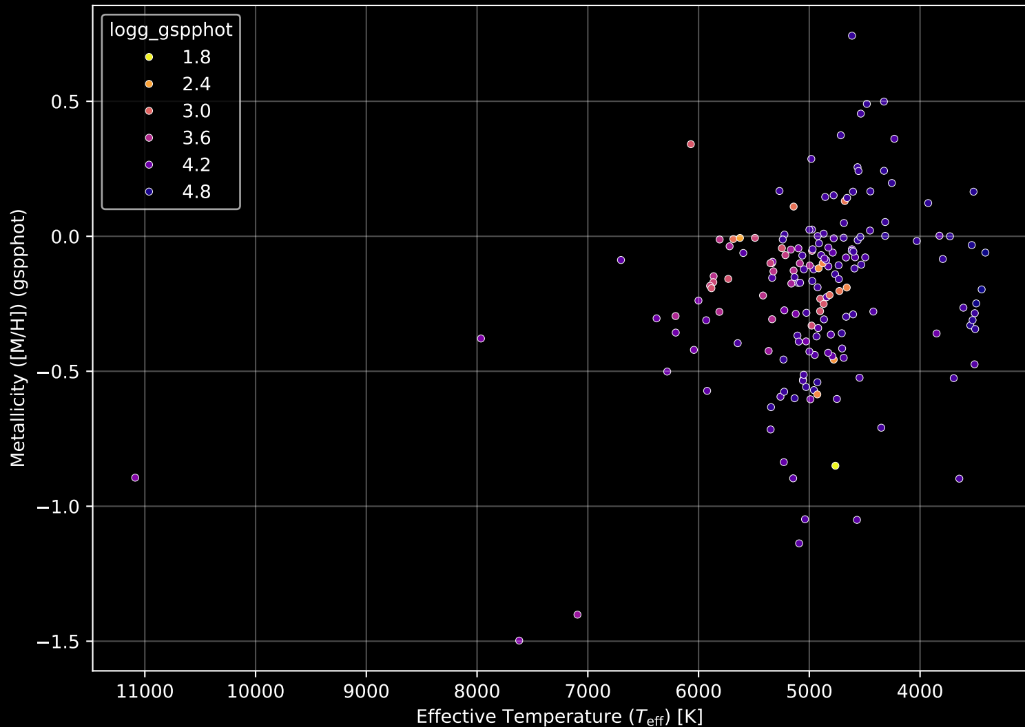
APOGEE DR17 Field: [K2_C8_130-53_btx] Stellar Population Parameters (n= 177)
