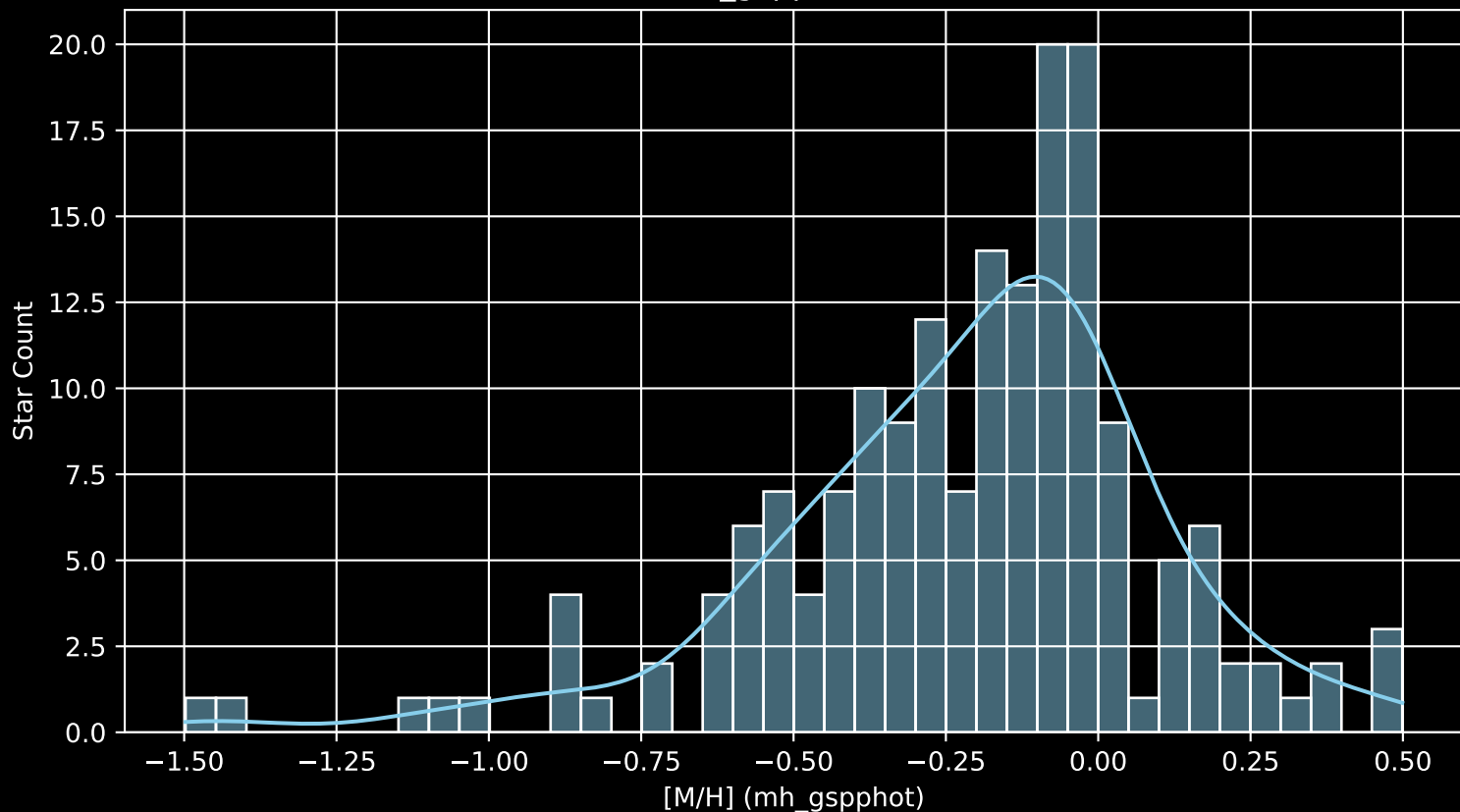
APOGEE DR17 Field: [K2_C8_130-53_btx [M/H] (mh_gspphot) (n= 176)
