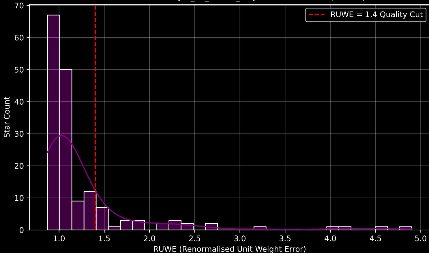
GAPOGEE DR17 Field [K2_C8_130-53_btx] RUWE Distribution (n= 166)
