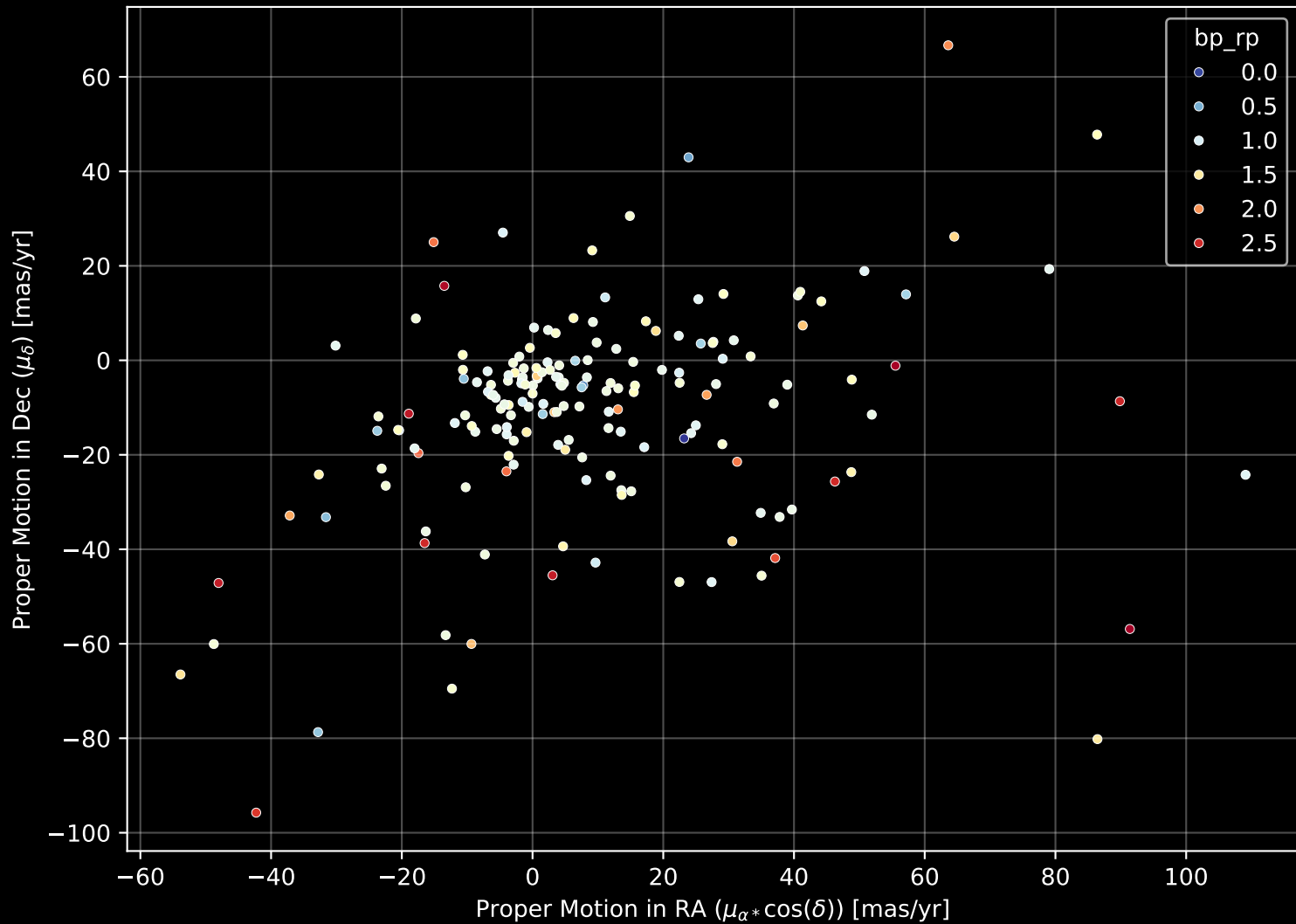
APOGEE DR17 Field: [K2_C8_130-53_btx] Proper Motion Diagram (n= 177)
