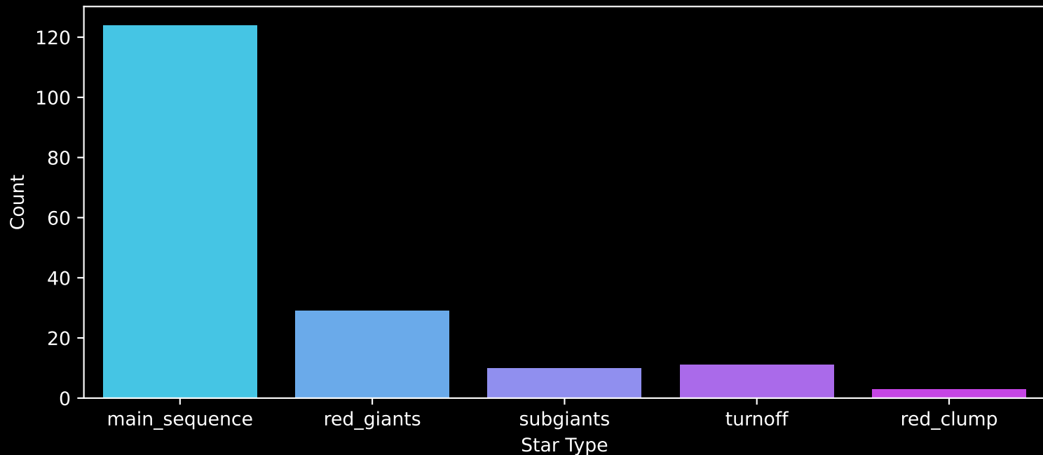
APOGEE DR17 Field: [K2_C8_130-53_btx] Count plot of Star Type
